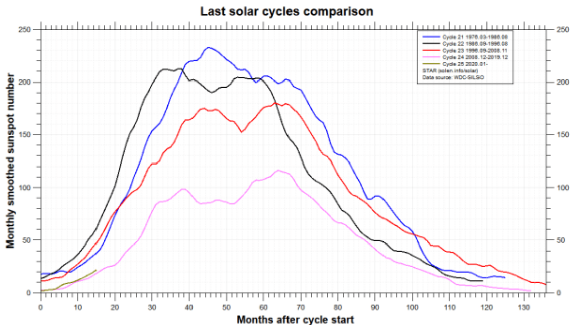
Solar Cycle 25 progression (green line) compared to 24, 23, 22 & 21 [updated Oct 1, 2021 — solen.info ] source Electrovease.
